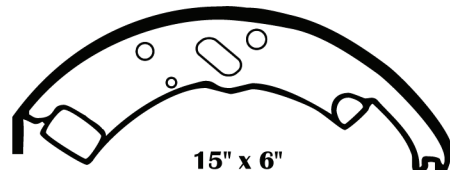
15" x 6" FMSI LINING 4596
