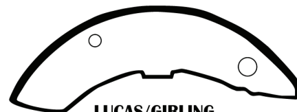
LUCAS/GIRLING 15" x 5" FMSI LINING 4528A
